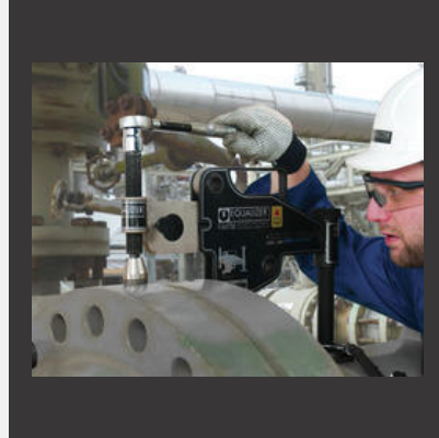
Fa4tm Flange Alignment Tool
