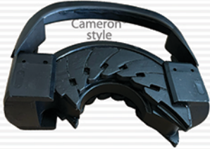
VBR Packers and Top Seals
